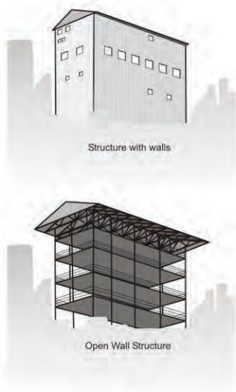
Figure 4-18. Drawing of a conventional and an open structure with a protective overhang.
