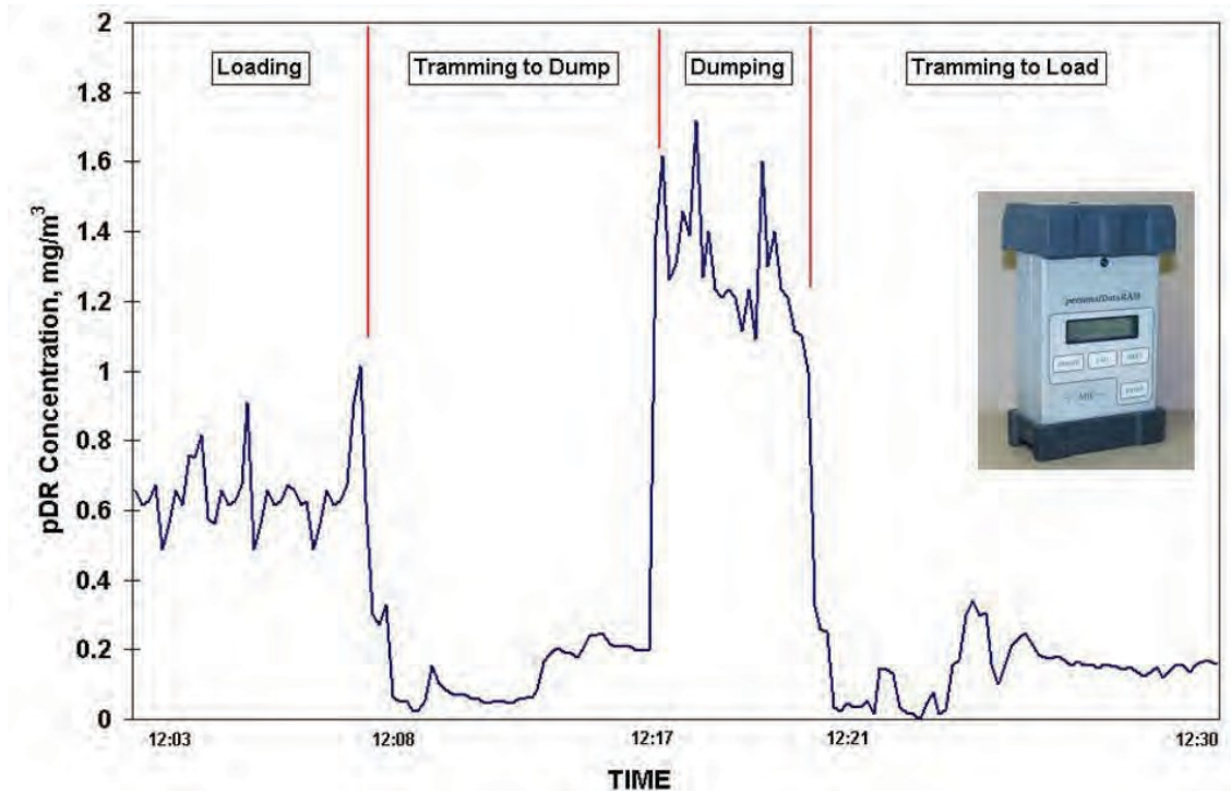
Figure 2-2. Example of dust measurements obtained with pDR.
