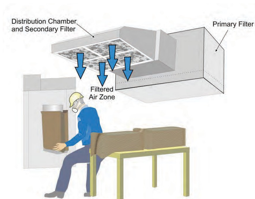
Figure 4-19 - Overhead air supply island system.
