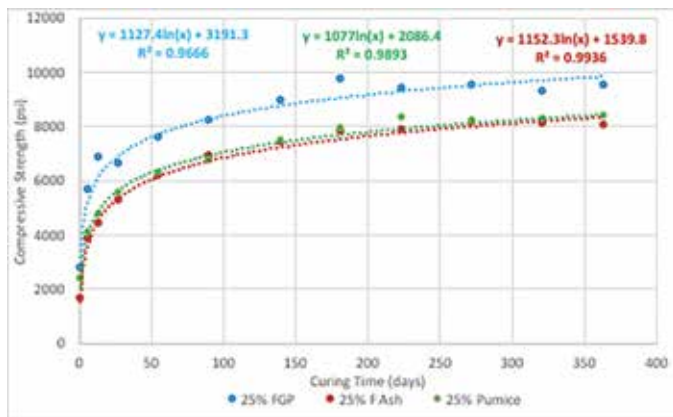
Figure 2: Compressive Strength Development of 25% Substitution Mixtures
