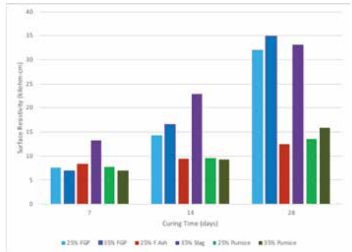
Figure 4: Surface Resistivity Development from 7 to 28 Days
