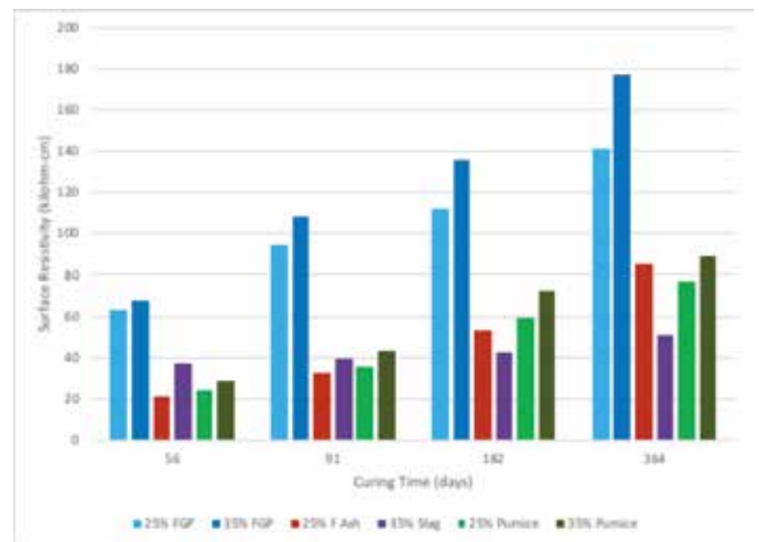
Figure 5: Surface Resistivity Development from 56 to 364 Days
