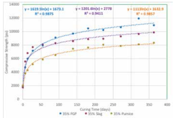
Figure 3: Compressive Strength Development of 35% Substitution Mixtures
