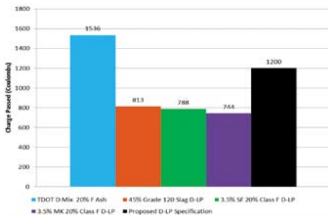
Figure 3. Comparison of D-LP and Class D Rapid Chloride Permeabilities
