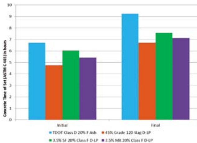
Figure 7. Comparison of D-LP and Class D ASTM C 403 Times of Set
