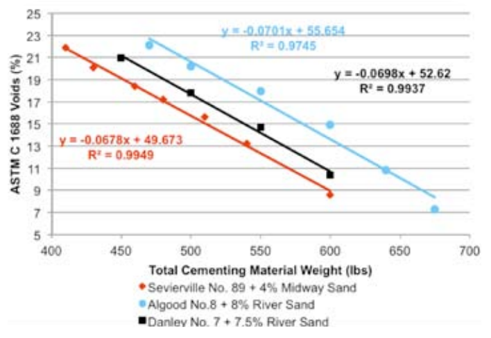
Figure 6: Plastic Voids (ASTM C 1688) vs. Cementing Materials for Constant w/cm
