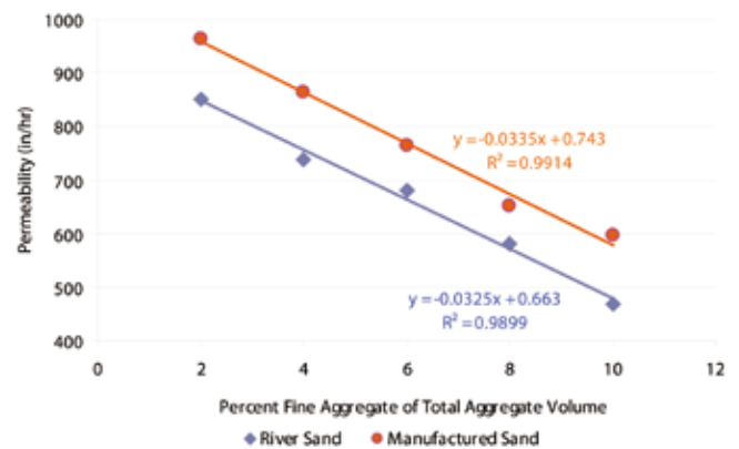
Figure 3. Permeability vs. Percent Fine Aggregate
