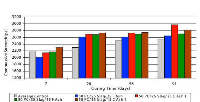
Figure 7. Compressive Strength Development of Tertiary Mixtures
