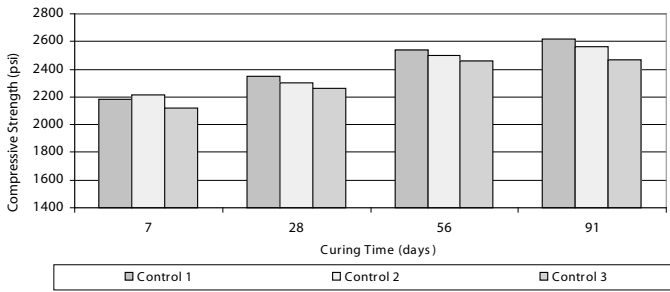
Figure 2. Control Mixture Compressive Strength Development
