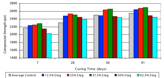
Figure 6. Compressive Strength Development of Grade 120 Slag Cement Mixtures
