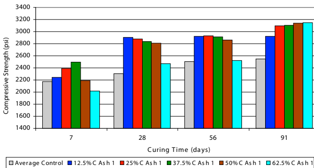
Figure 4. Compressive Strength Development of Class C Fly Ash Number 1 Mixtures
