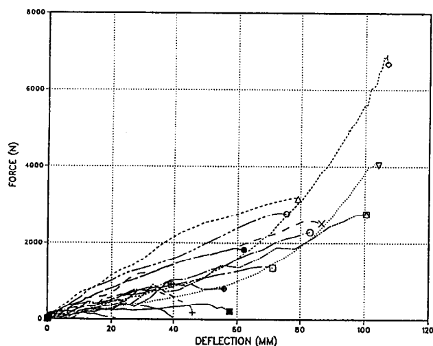
FIGURE 14. Lap belt impactor, frontal response of the lower abdomen. (From Rouhana et al. 15 , 1989. Reprinted with permission from Society of Automotive Engineers, Inc.)
