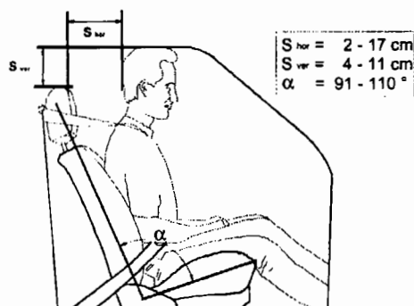
Fig. 4 Initial position in the car seat
