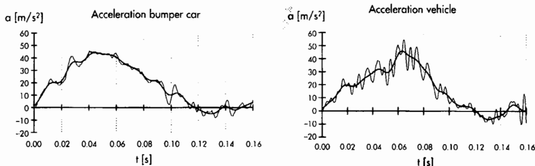
Fig. 10 Comparison of the acceleration signals from the bumper car (left) and automobile (right)
