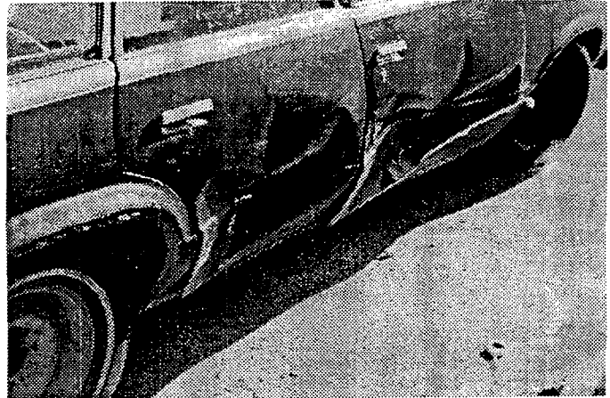
Figure 30. Chevrolet Malibu lateral impact. Energy absorption by door was approximately 900 Joules (forward door). Dent is 102 mm deep.
