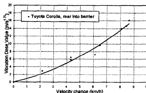
Figure 44. Comparison of VDV and \Delta V for rear-end impacts.
