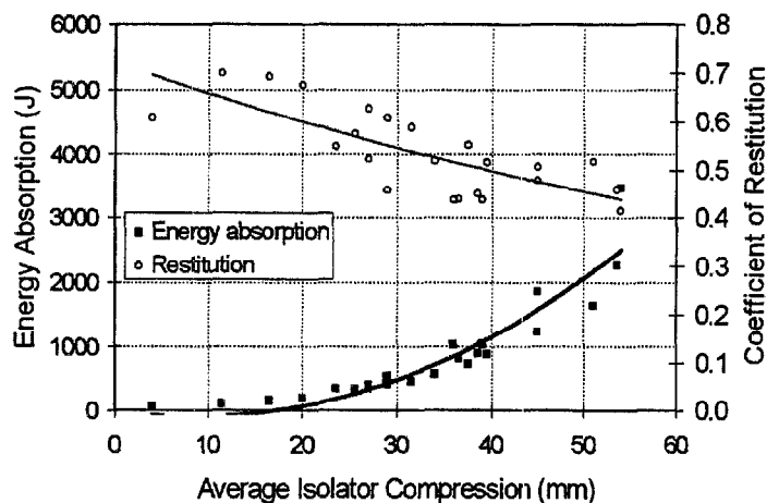
Figure 8. VW rear vehicle-to-barrier data.
