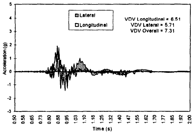
Figure 36. Acceleration for test SS10. Damage at right.
