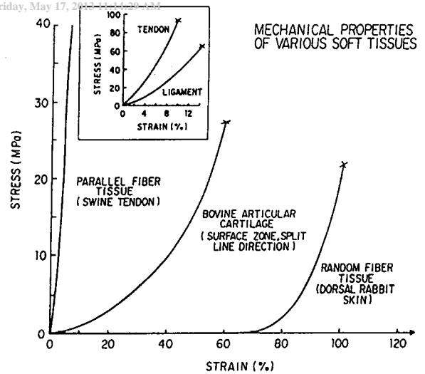
FIGURE 15. Typical stress-strain curves for various soft tissues. (From Woo et al. 16 )
