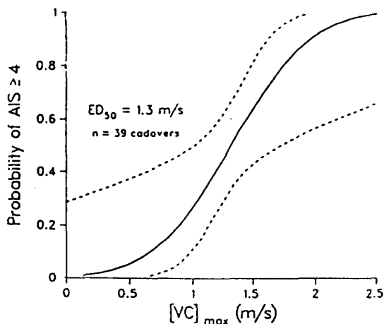
FIGURE 10. Curve showing the probability of thoracic AIS >3 as a function of VC max . These data were derived from unembalmed cadaver impacts run at University of California, San Diego. (From Viano and Lau 10 , 1986. Reprinted with permission from Society of Automotive Engineers, Inc.)
