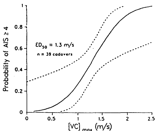
FIGURE 10. Curve showing the probability of thoracic AIS >3 as a function of VC_{max} . These data were derived from unembalmed cadaver impacts run at University of California, San Diego. (From Viano and Lau 10 , 1986. Reprinted with permission from Society of Automotive Engineers, Inc.)
