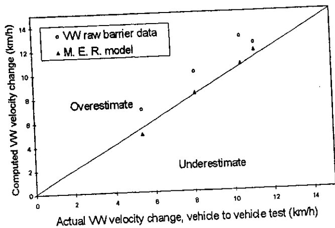
Figure 10. Actual and computed \Delta V , vehicle-to-vehicle impacts.
