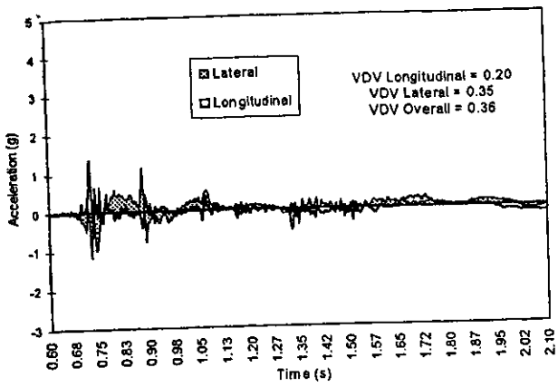
Figure 39. Acceleration for test SS13. Damage at right.
