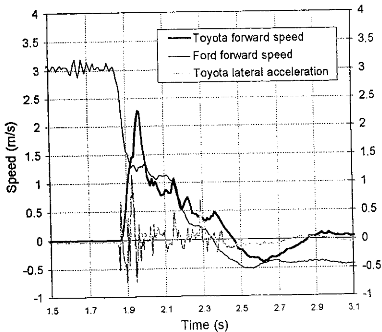
Figure 22. Speed and acceleration for test 4. Damage right rear door and B-pillar.
