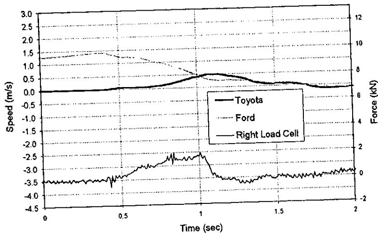
Figure 33. Speed and force for test 23. Damage at right.
