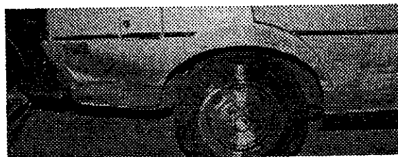
Dent in quarter panel 11 cm farther forward than test 19, plus small dent in wheel arch leading edge.
