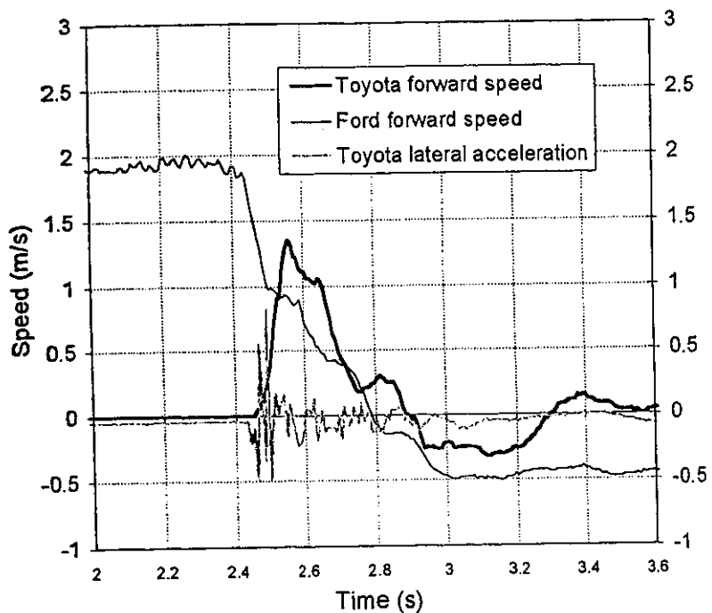
Figure 21. Speed and acceleration for test 3. Additional damage to lower right front door. Same area was damaged in test 2.
