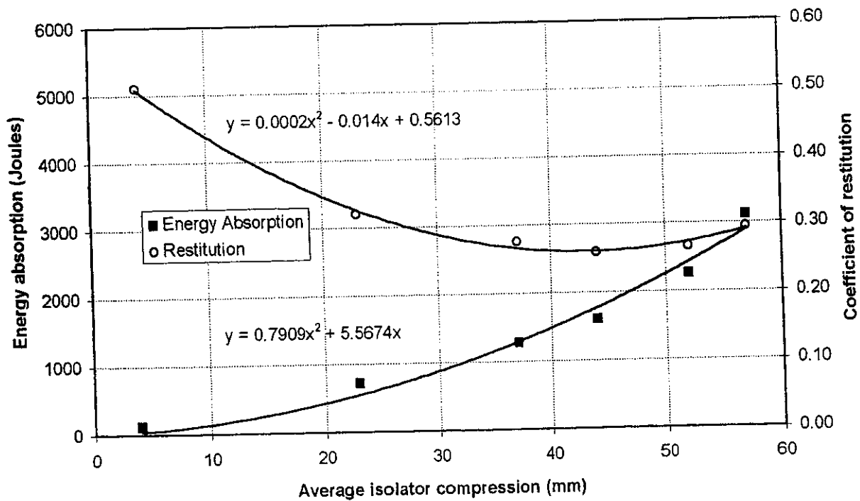
Figure 14. 1982 Ford Escort, 225 kg added (1134 kg).
