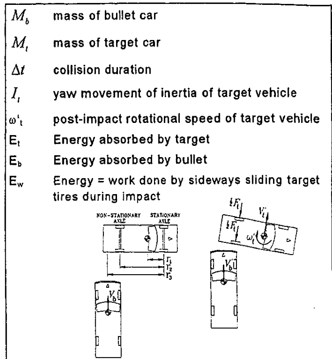
Figure 28. Nomenclature for lateral collision model.
