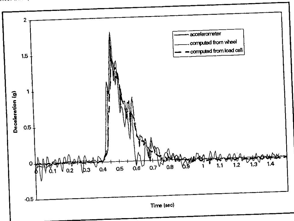
Figure 3. Comparison of vehicle acceleration from three sources: 5th wheel, accelerometer and load cells.
