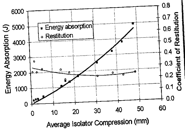
Figure 9. Granada front vehicle-to-barrier data.
