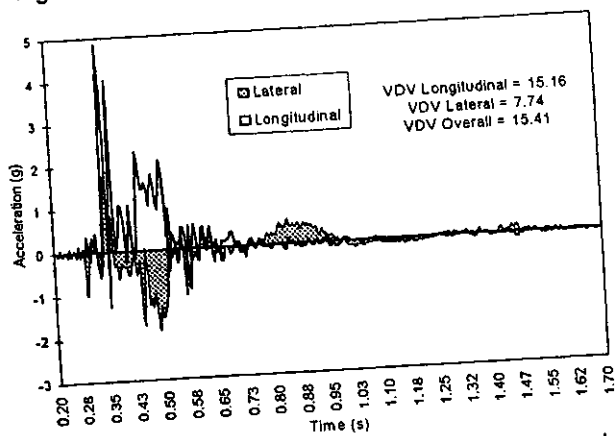
Figure 37. Acceleration for test SS11. Damage at right.
