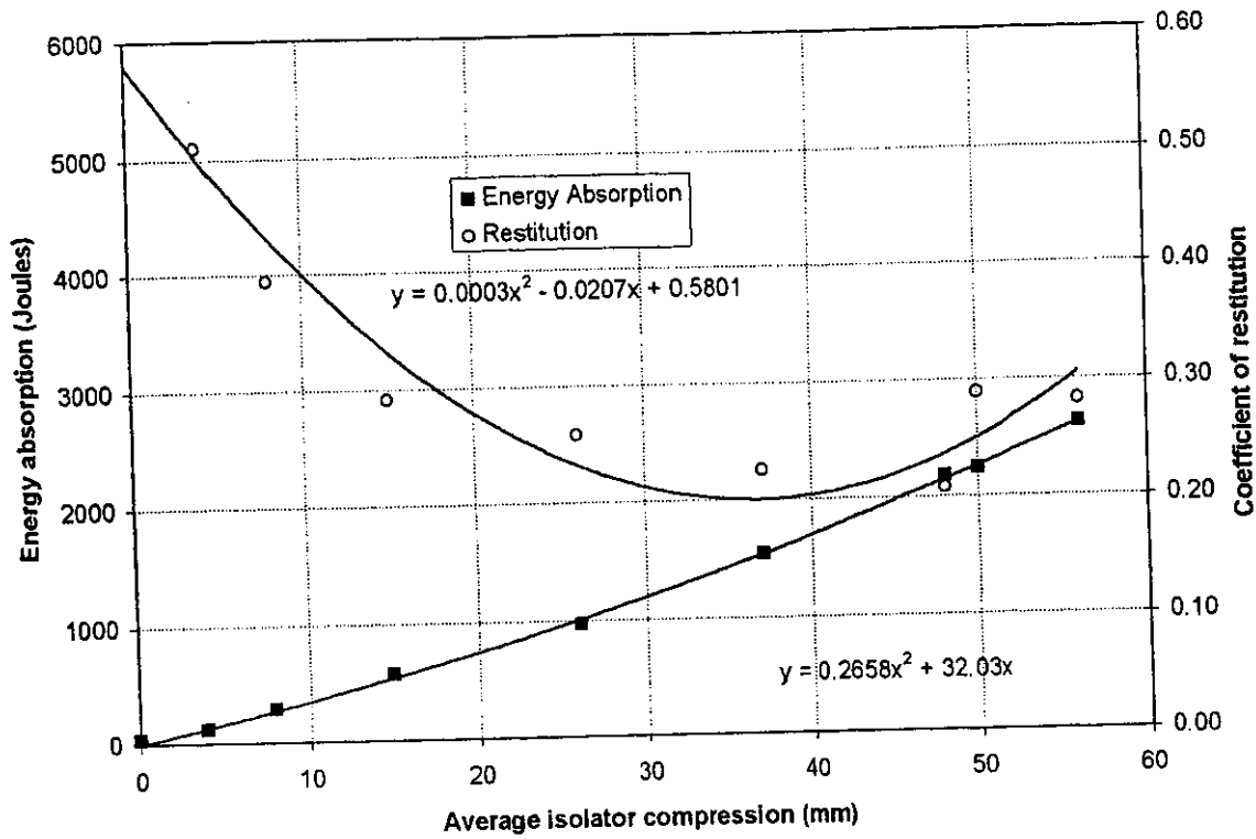
Figure 15. 1982 Ford Escort, 450 kg added (1359 kg).
