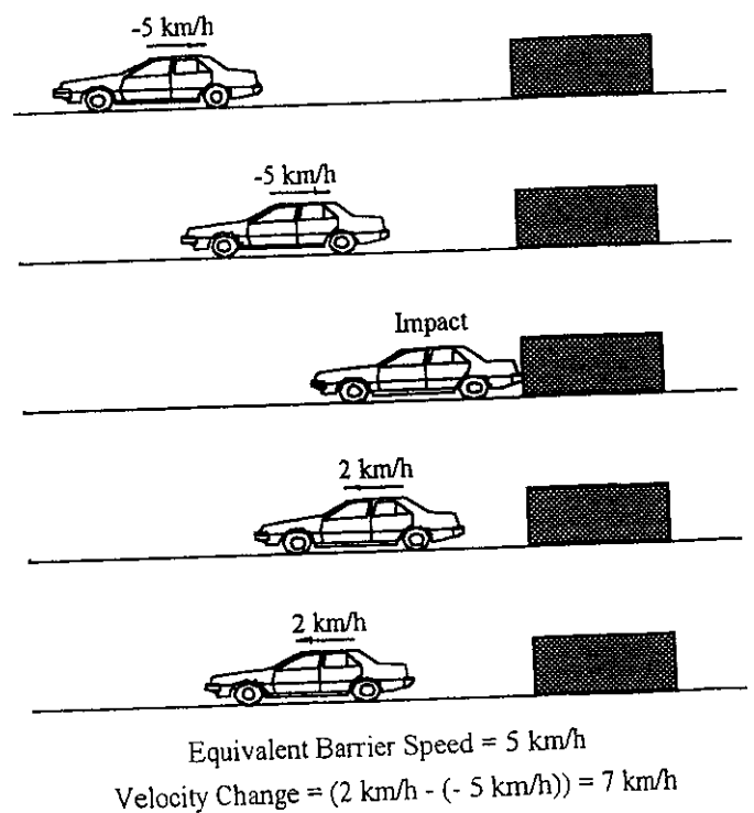
Figure 5. Equivalent barrier speed.
