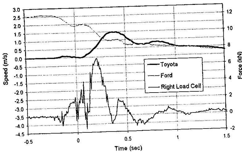
Figure 34. Speed and force for test 24. Damage at right.
