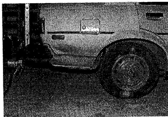
Dent in quarter panel, 200 mm diameter, 18 mm maximum depth.
