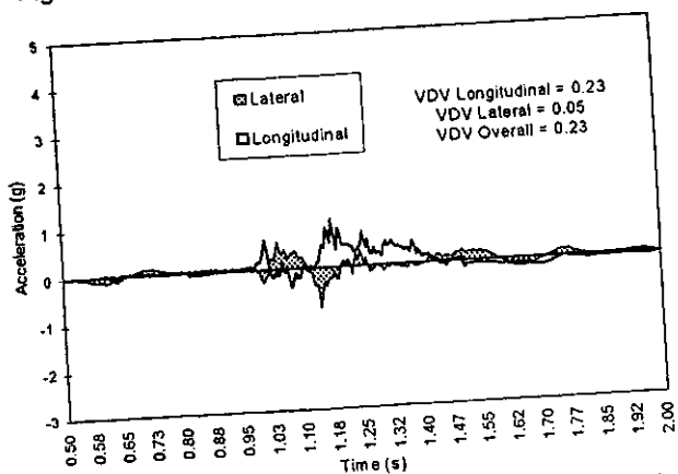
Figure 38. Acceleration for test SS12. Damage at right.
