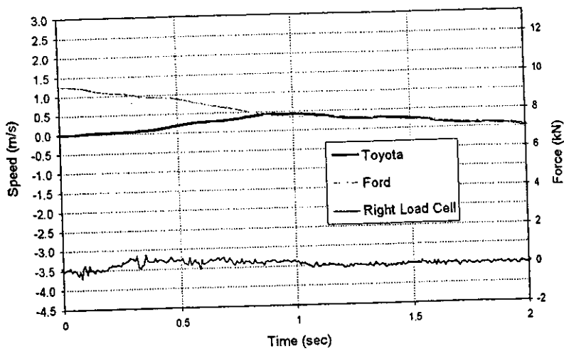
Figure 32. Speed and force for test 22. Damage at right.
