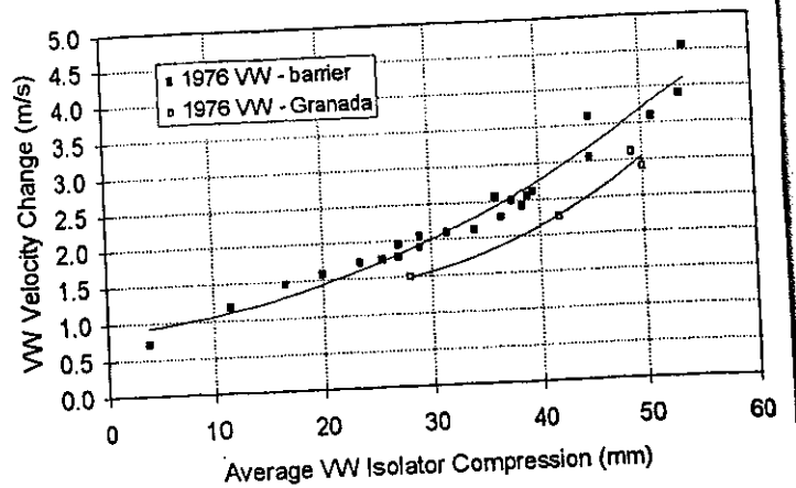
Figure 7. Average isolator compression, barrier and vehicle-to-vehicle impacts.
