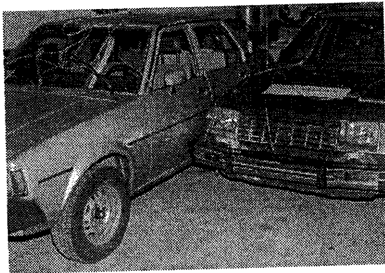
Figure 31. Vehicle engagement for side-swipe tests.
