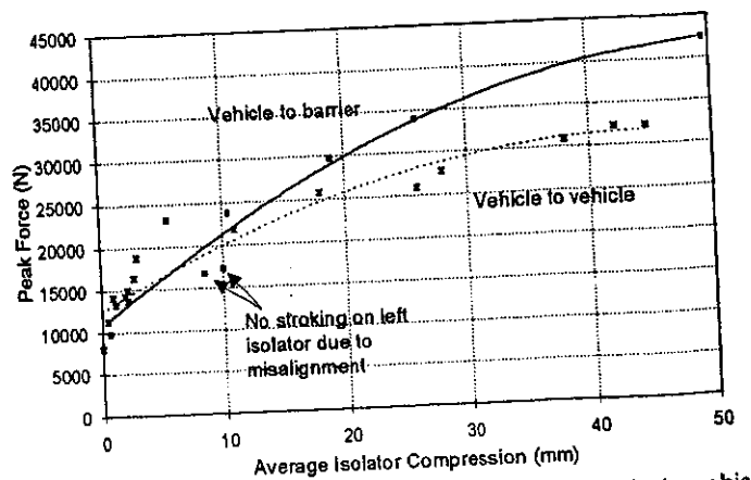
Figure 11. Escort front vehicle-to-barrier and vehicle-to-vehicle data.
