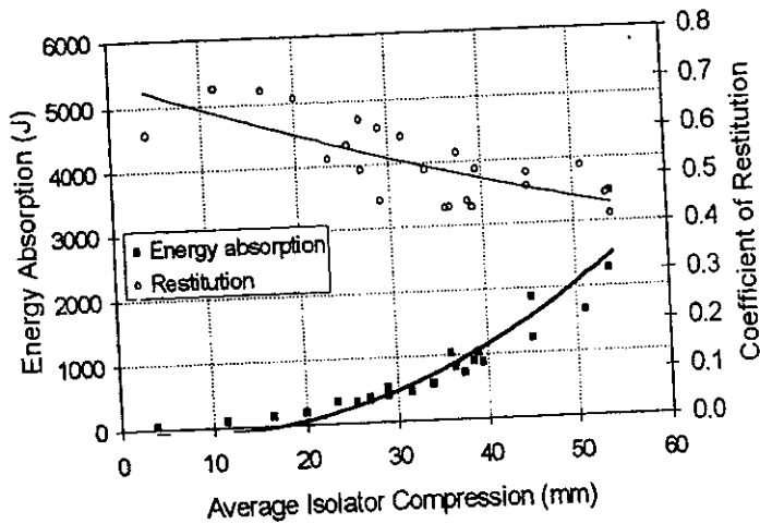
Figure 8. VW rear vehicle-to-barrier data.
