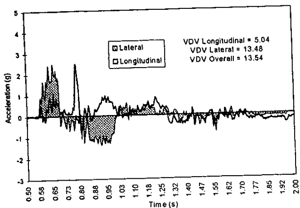
Figure 42. Acceleration for test SS19. Damage at right*.
