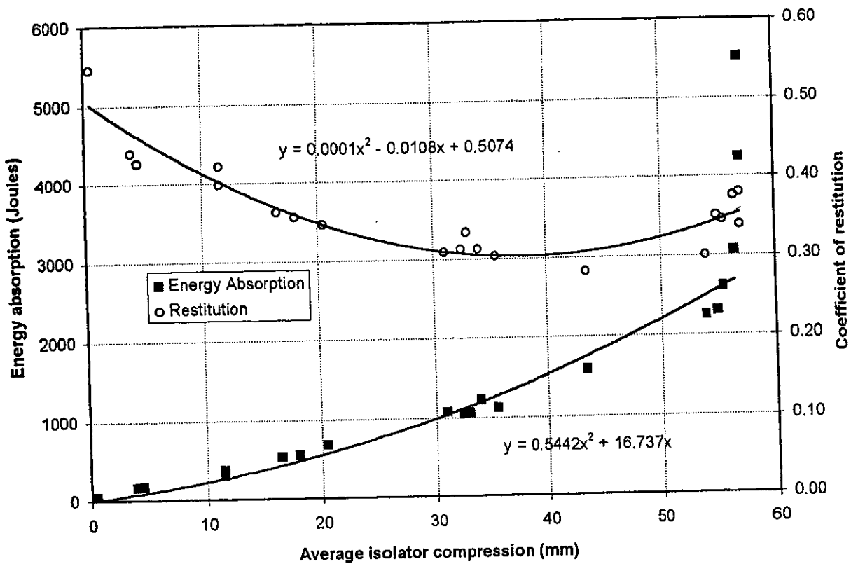
Figure 13. 1982 Ford Escort, empty (909 kg).
