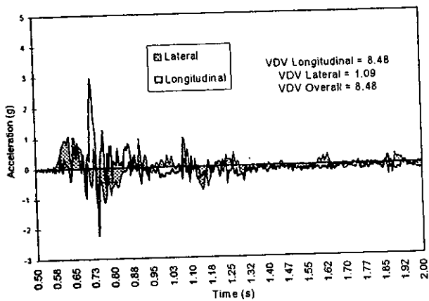
Figure 41. Acceleration for test SS18. Damage at right*.
