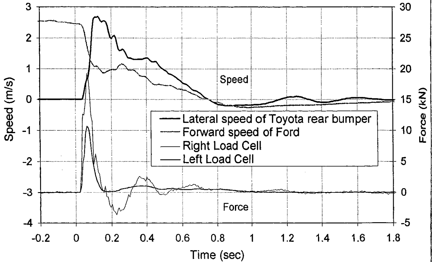
Figure 27 (a). Speed and force data for test 21.
