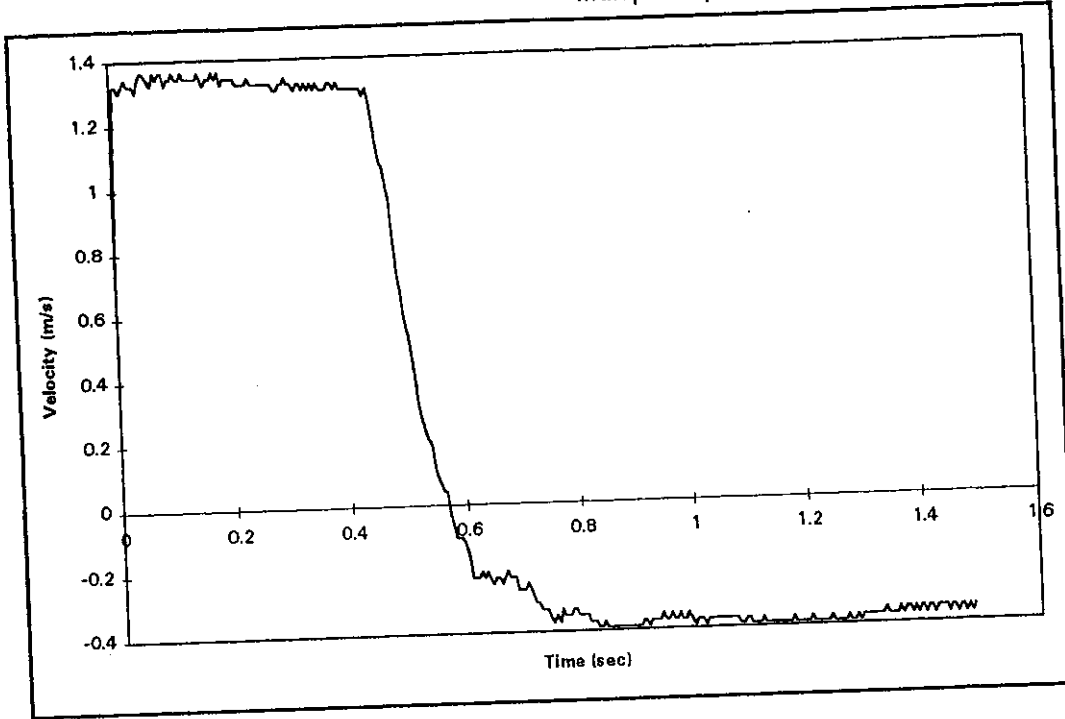
Figure 2. 5th Wheel trace, vehicle-to-barrier collision. The speed drops below zero when the vehicle rebounds backwards from the barrier.
