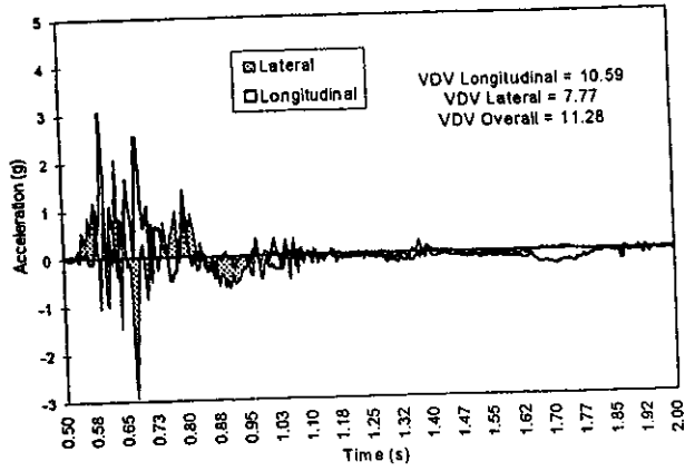
Figure 40. Acceleration for test SS17. Damage at right*.
