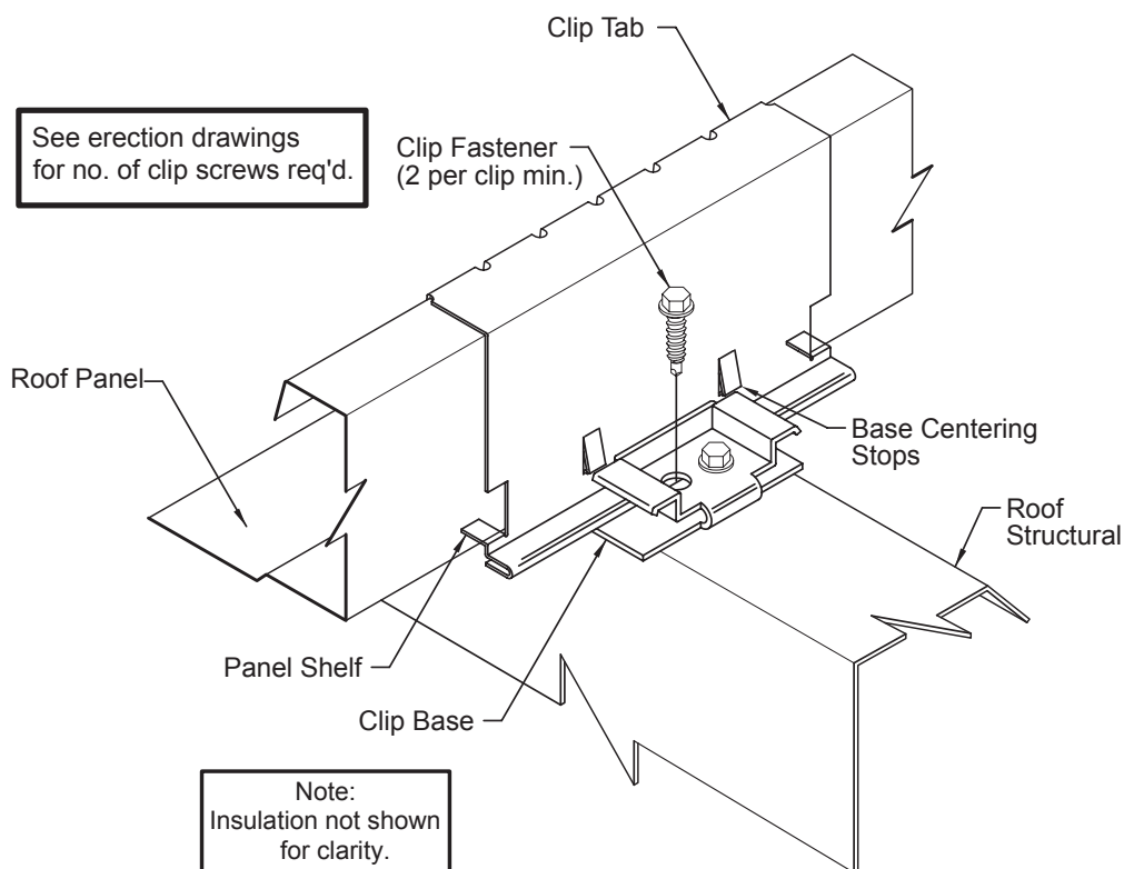
CLIP TO PANEL ASSEMBLY
