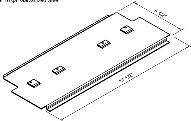
Part No. BP-218 Weight - 2.21
