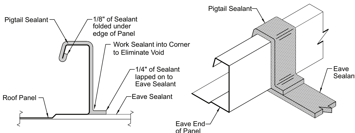
EAVE PIGTAIL SEALANT DETAIL
