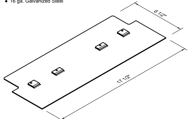
Part No. BP-218-0 Weight - 1.86
