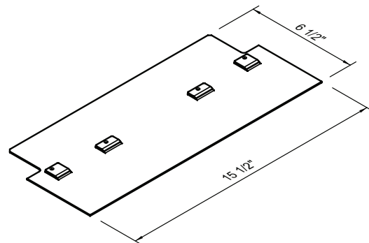
Part No. BP-216-0 Weight - 1.64
