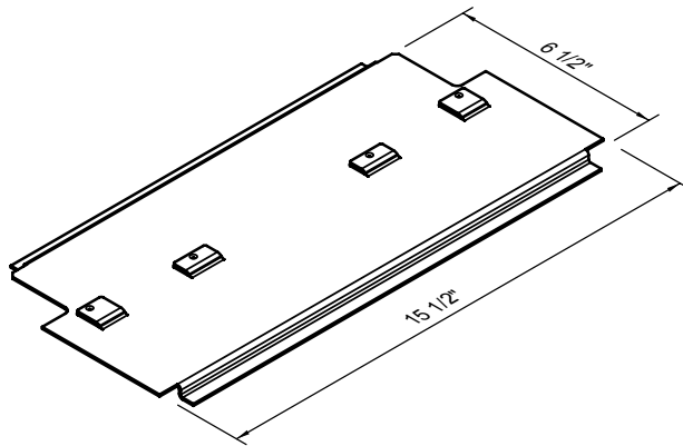
Part No. BP-216 Weight - 1.94
