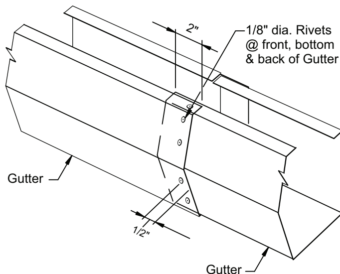
EAVE GUTTER SPLICE
