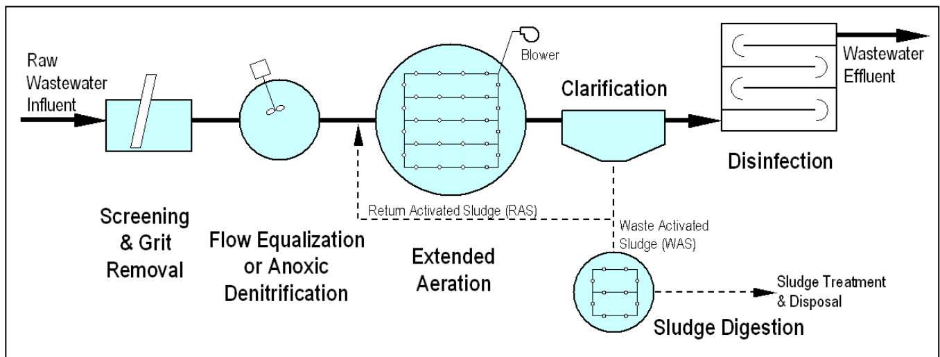
Figure 6 -- Extended Aeration Activated Sludge Process Flow Schematic
