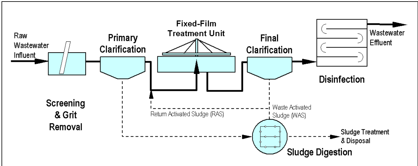
Figure 8 – Fixed Film Process Flow Schematic
