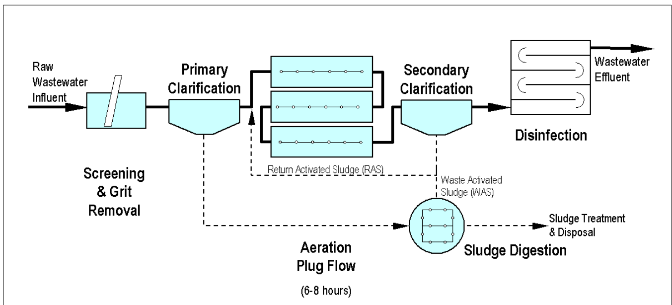
Figure 5 -- Conventional Activated Sludge Process Flow Schematic
