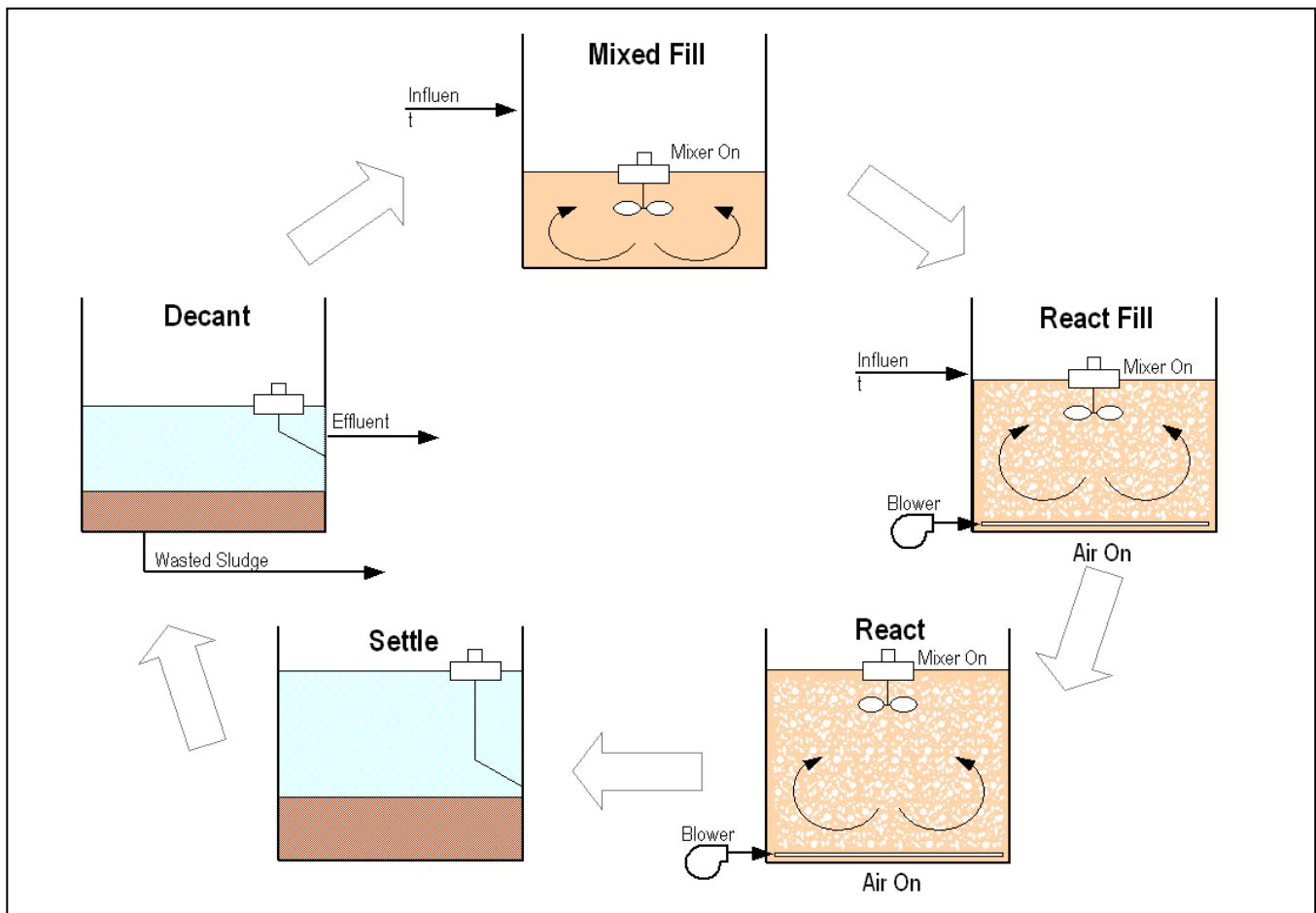
Figure 10 –SBR Batch Operation Sequence
