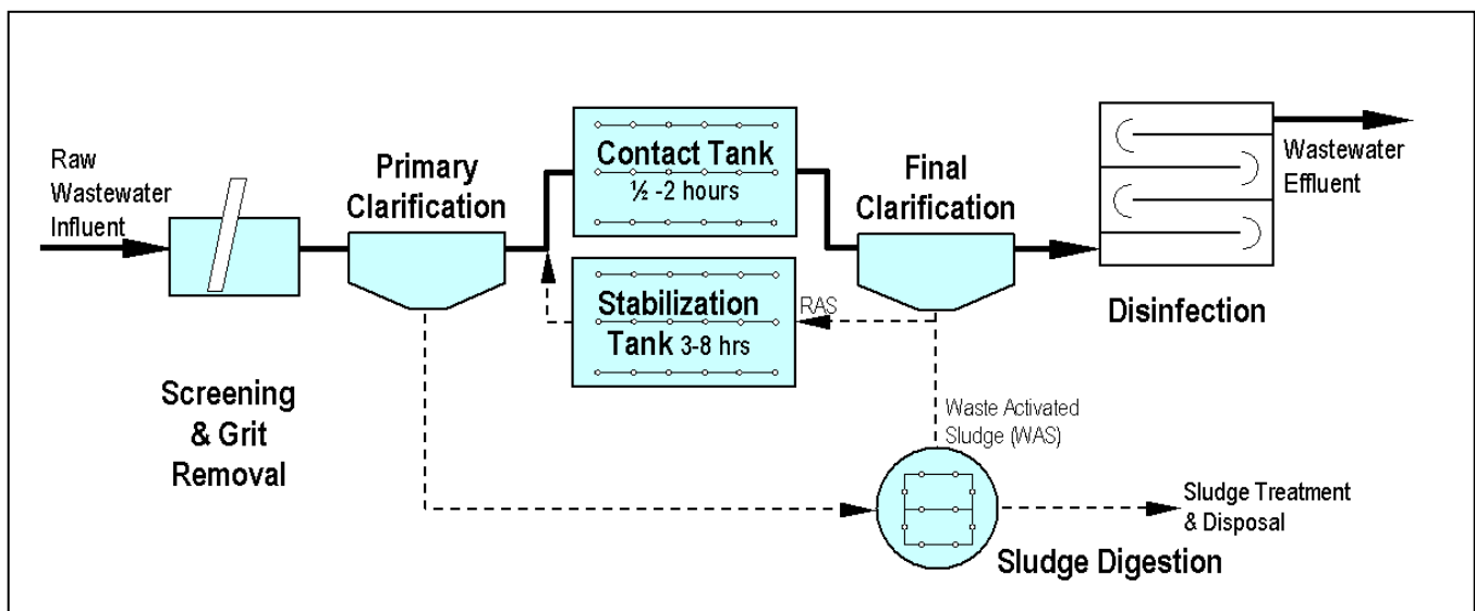
Figure 7 -- Contact Stabilization Suspended Growth Process Flow Schematic
