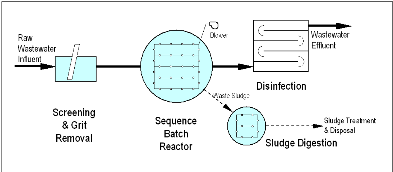
Figure 9 – Sequence Batch Reactors (SBRs) Process Flow Schematic
