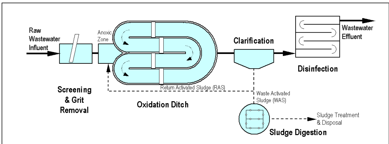
Figure 2 ~ Oxidation Ditches Process Flow Schematic
