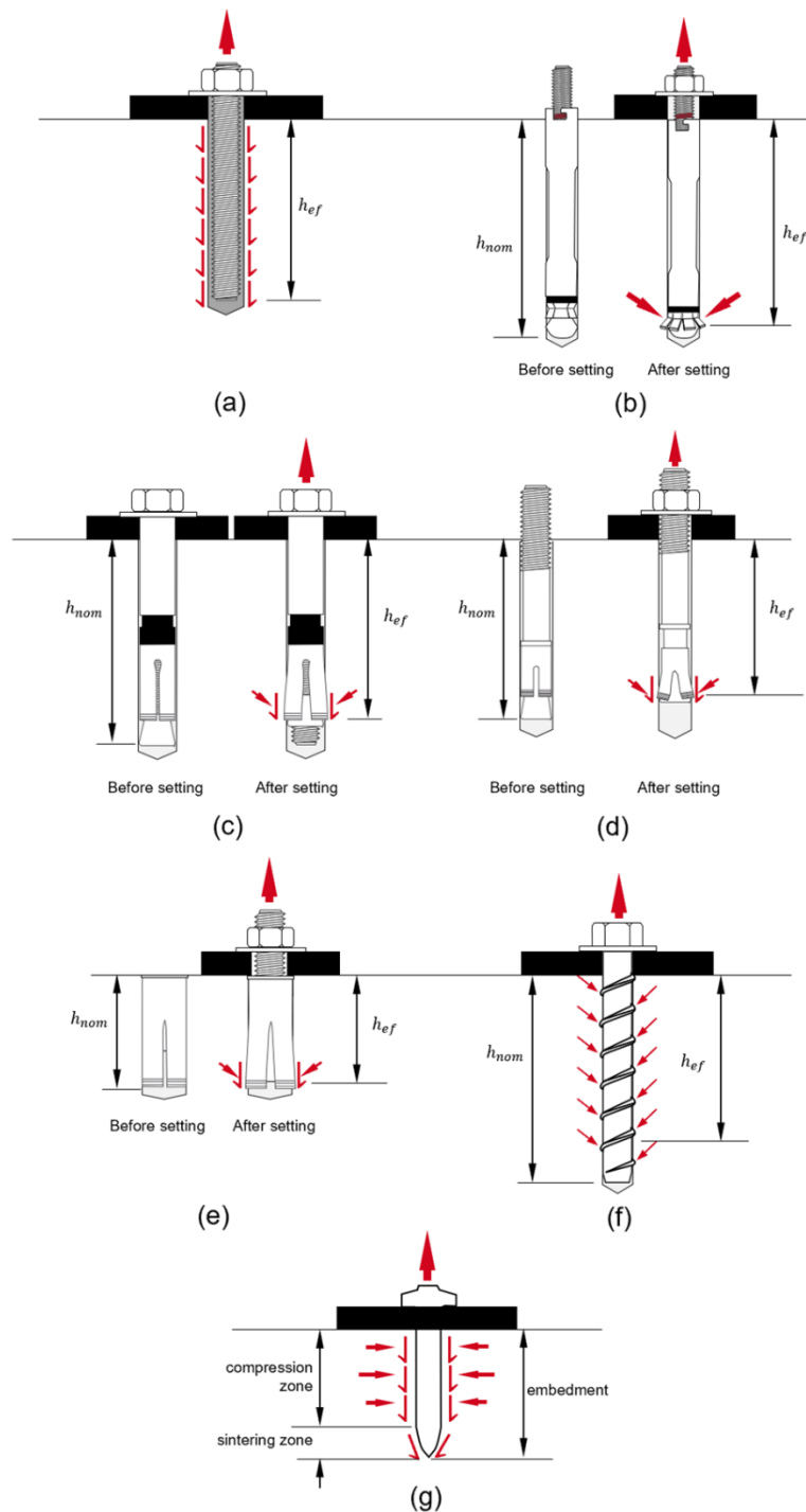
Figure 1. (a) adhesive anchor, (b) undercut anchor, (c) sleeve-type torque-controlled expansion anchor, (d) stud-type torque-controlled expansion anchor, (e) displacement-controlled expansion anchor, (f) screw anchor, (g) power-actuated fasteners
