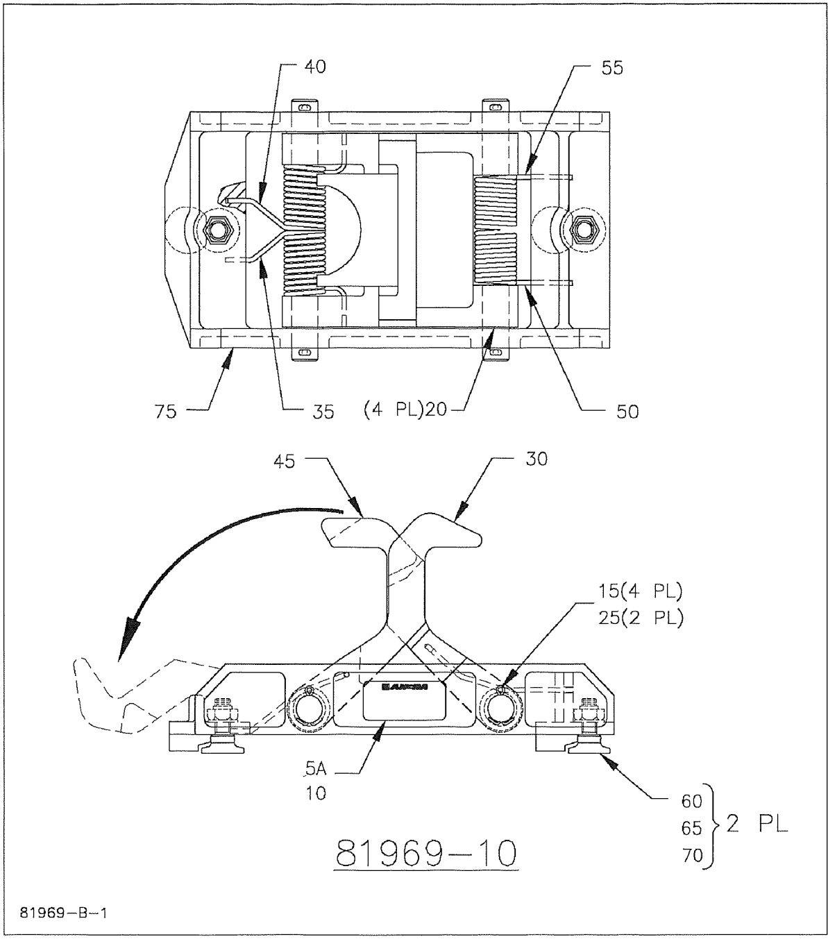
Cargo Lock Assembly, PN 81969-10 Figure 14
