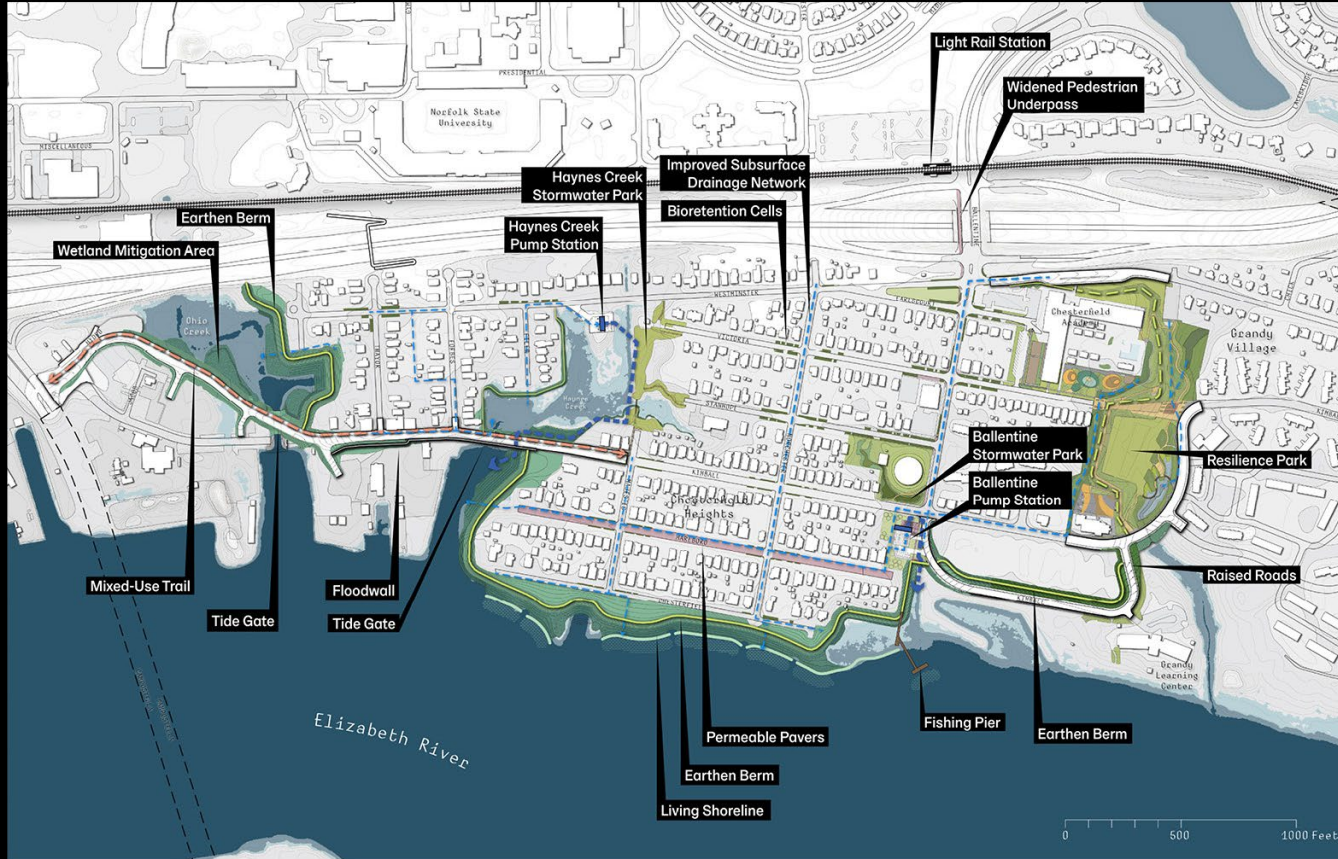
Levees & Floodwalls
