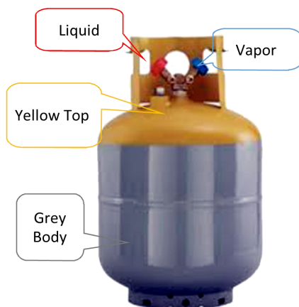
Figure 12. Recovery Tank.
