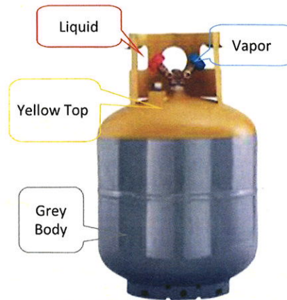
Figure 12. Recovery Tank.
