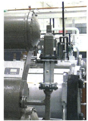
Figure 18. Rupture Disc.
