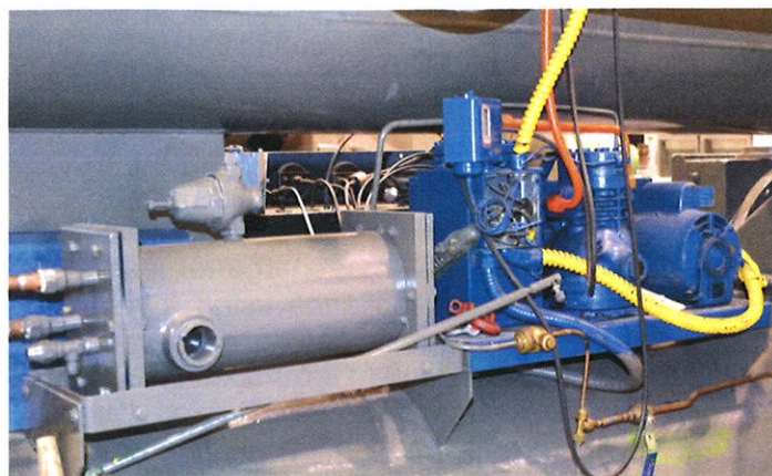
Figure 16. Purge Unit.
